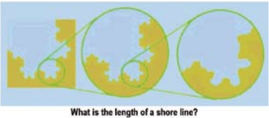
What is the length of a shore line?
